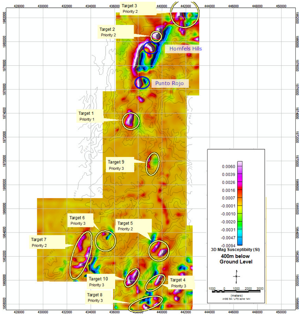
Target Areas on Susceptibility Model at 400m depth
