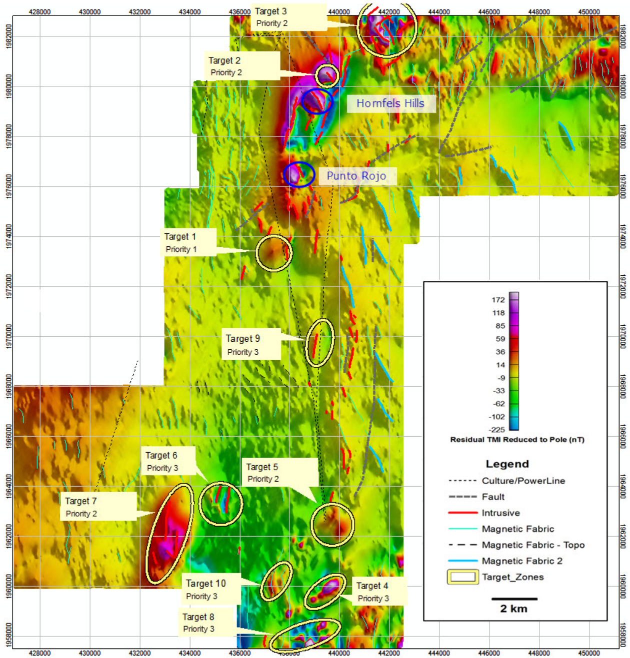
Target Areas on Residual Magnetics
